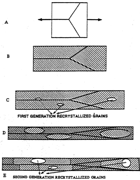
Fig. 6 Schematic illustration showing sequence of deformation-recrystallization steps in dynamic recrystallization.
